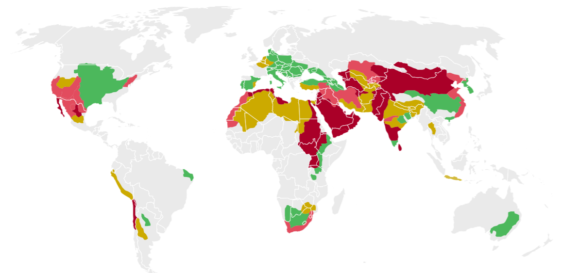
Figure 7: Northern Africa, Central Asia and the Middle East are the regions most prone to conflicts due to water scarcity in underlying water basins
